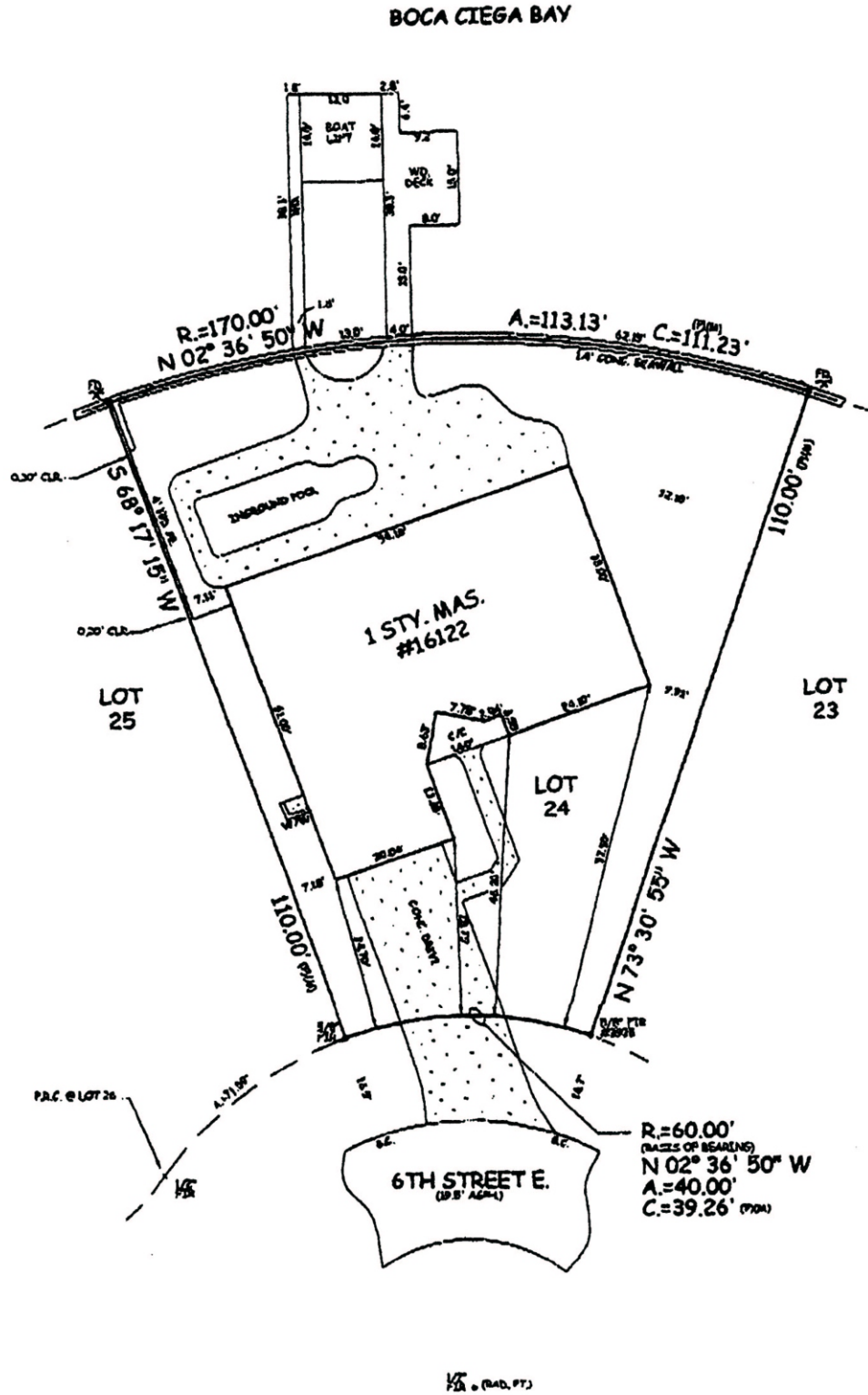
This image has been cropped from the full survey done by Murphy's Land Surveying, Inc., dated September 2003
