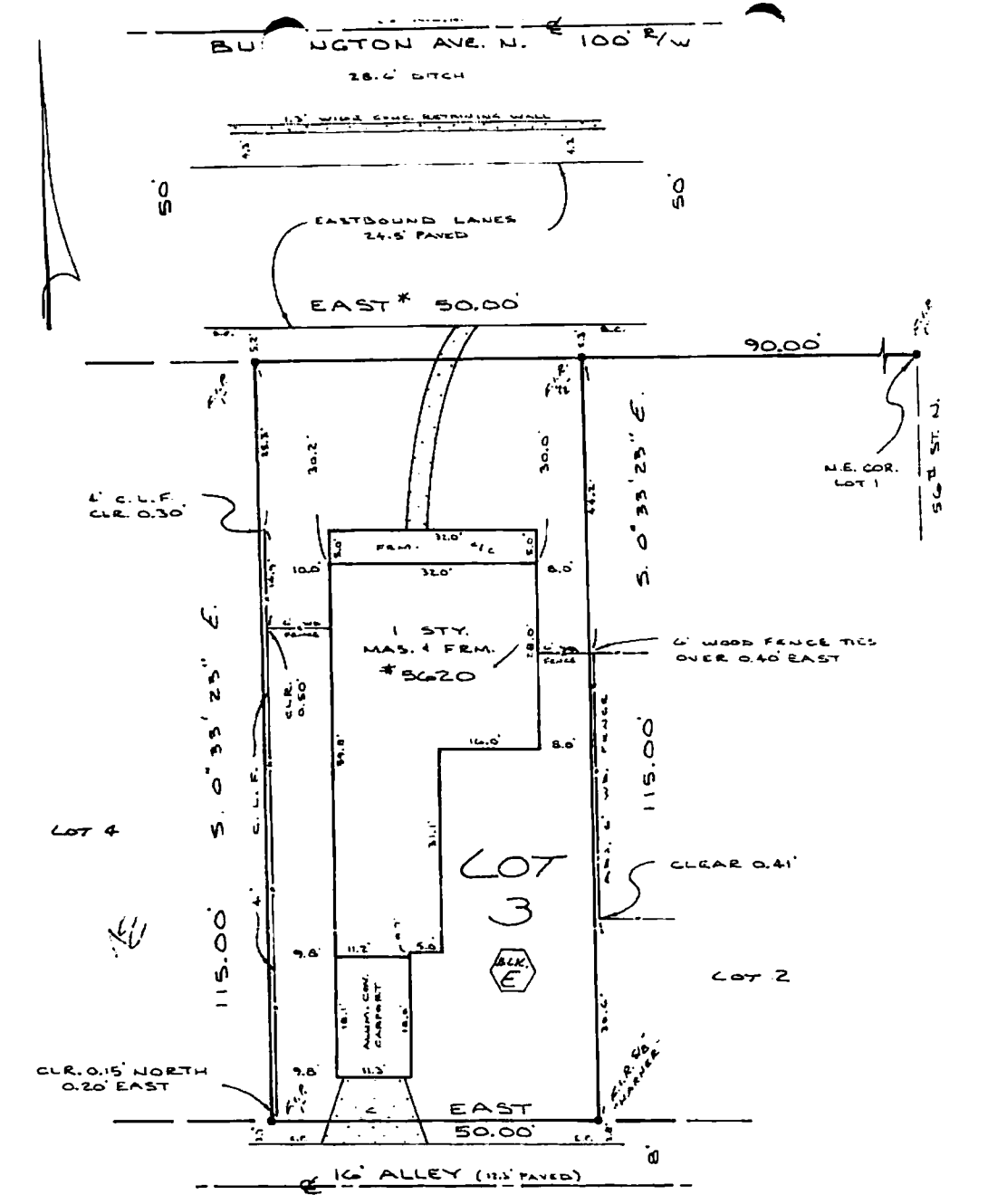
A BOUNDARY SURVEY OF: Lot 3, Block E, REVISED PLAT OF STONEMONT SUBDIVISION as recorded in Plat Book 6, Page 36 of the Public Records of Pinellas County, Florida.
